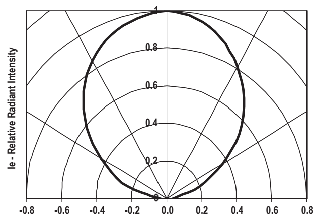
Figure 4. Angular Displacement Vs Relative Radiant Intensity
