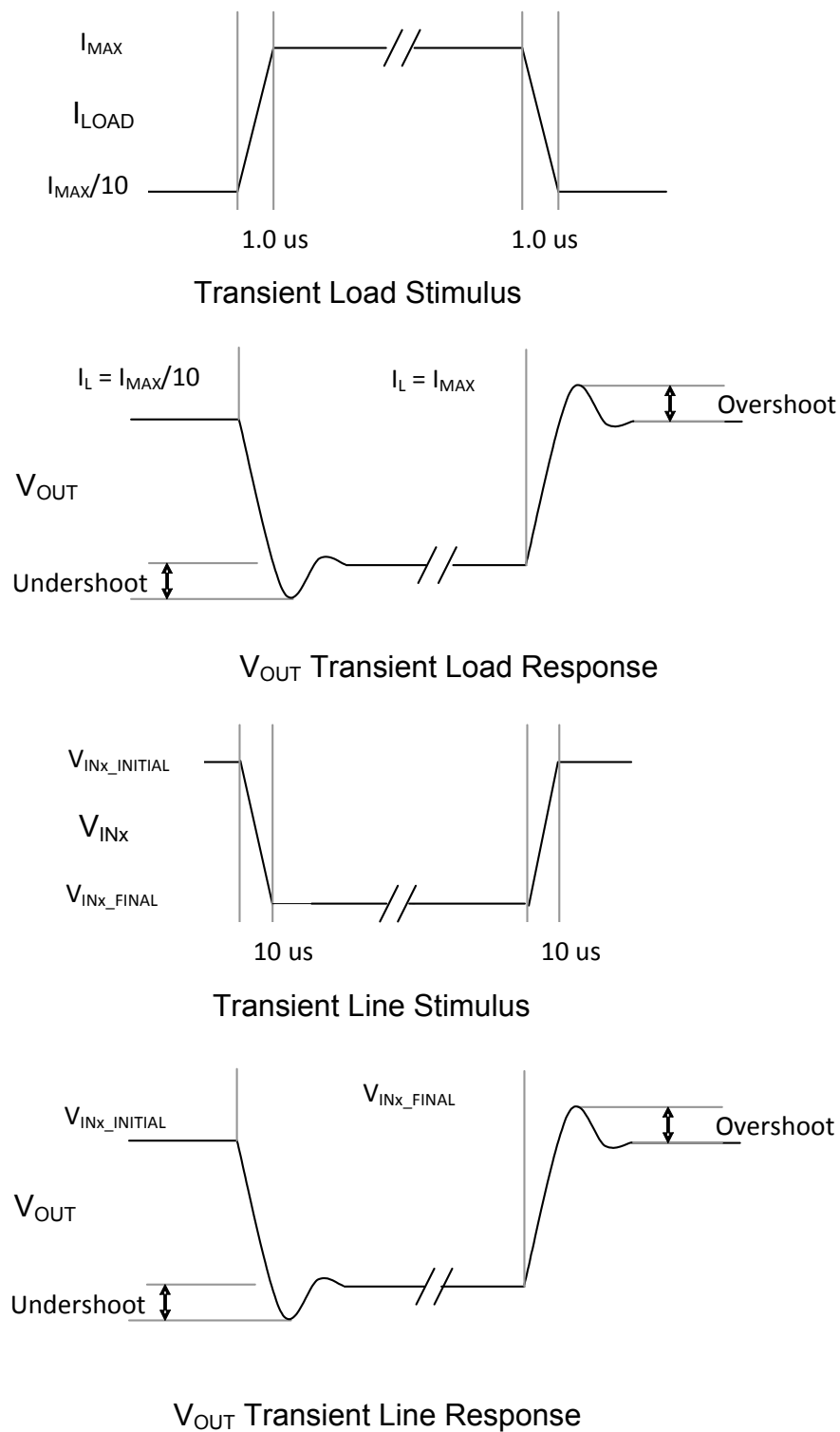
Figure 31. Transient Waveforms
