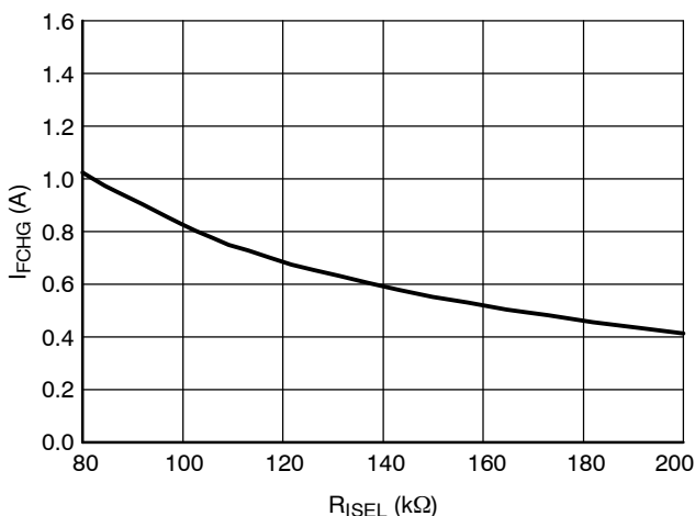
Figure 17. Full-Charge Current ( I_{\text{FCHG}} ) vs. Current Select Resistor ( R_{\text{ISEL}} )
