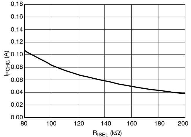
Figure 18. Pre-Charge Current ( I_{\text{PCHG}} ) vs. Current Select Resistor ( R_{\text{ISEL}} )
