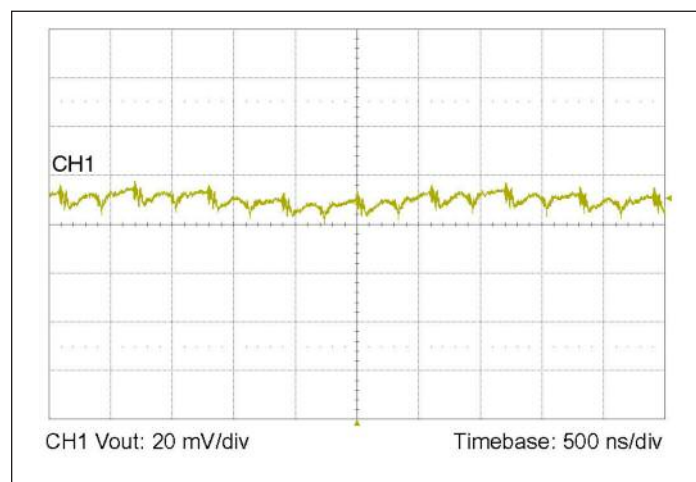
Figure 8 — Output voltage ripple at full load and 48 V_{IN} with 10 \mu\text{F} ceramic external bypass capacitor and 20 nH of distribution inductance.
