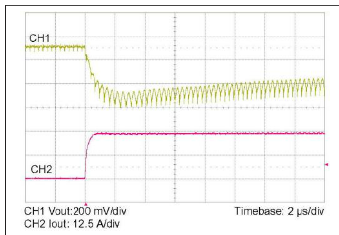
Figure 10 — 0 – 25 A load step with 100 \mu\text{F} input capacitor and no output capacitor.
