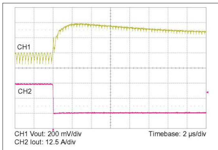
Figure 11 — 25 – 0 A load step with 100 \mu\text{F} input capacitor and no output capacitor.
