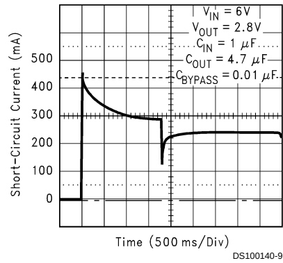
Short-Circuit Current
