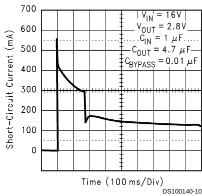
Short-Circuit Current
