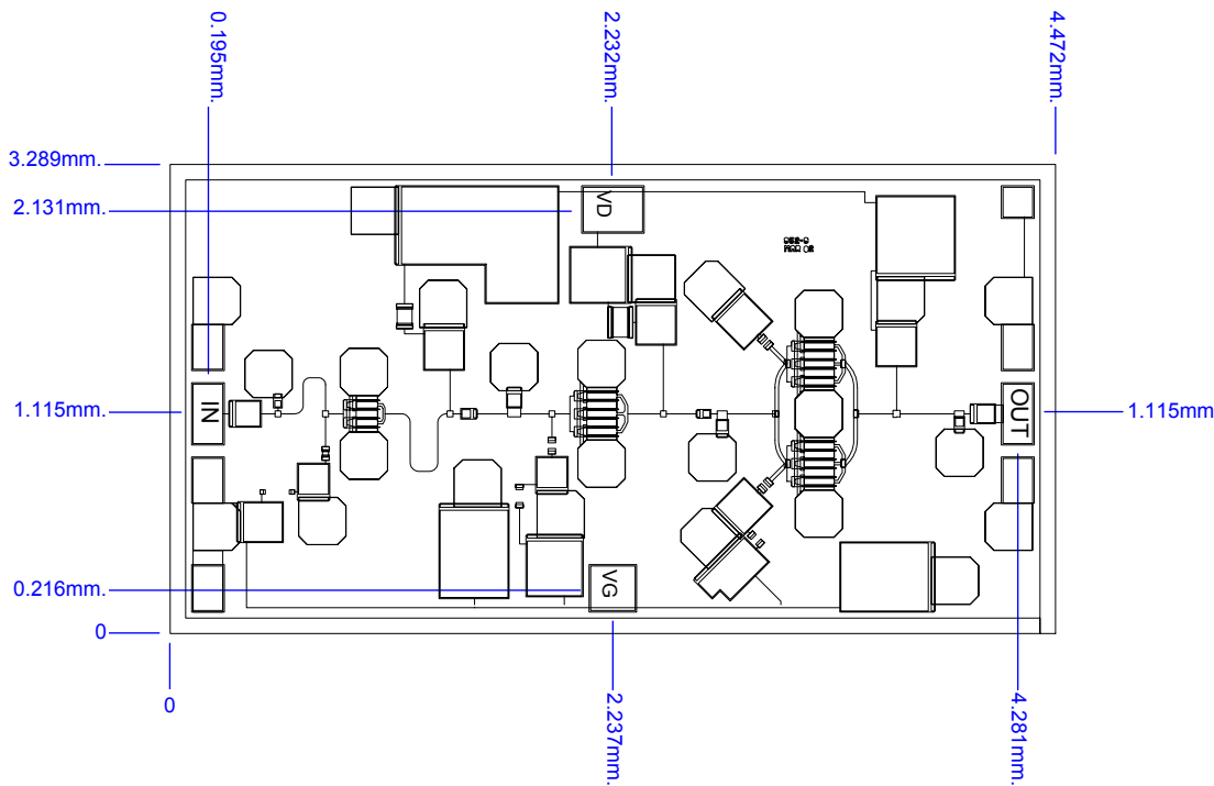
Figure 5. Die Layout
