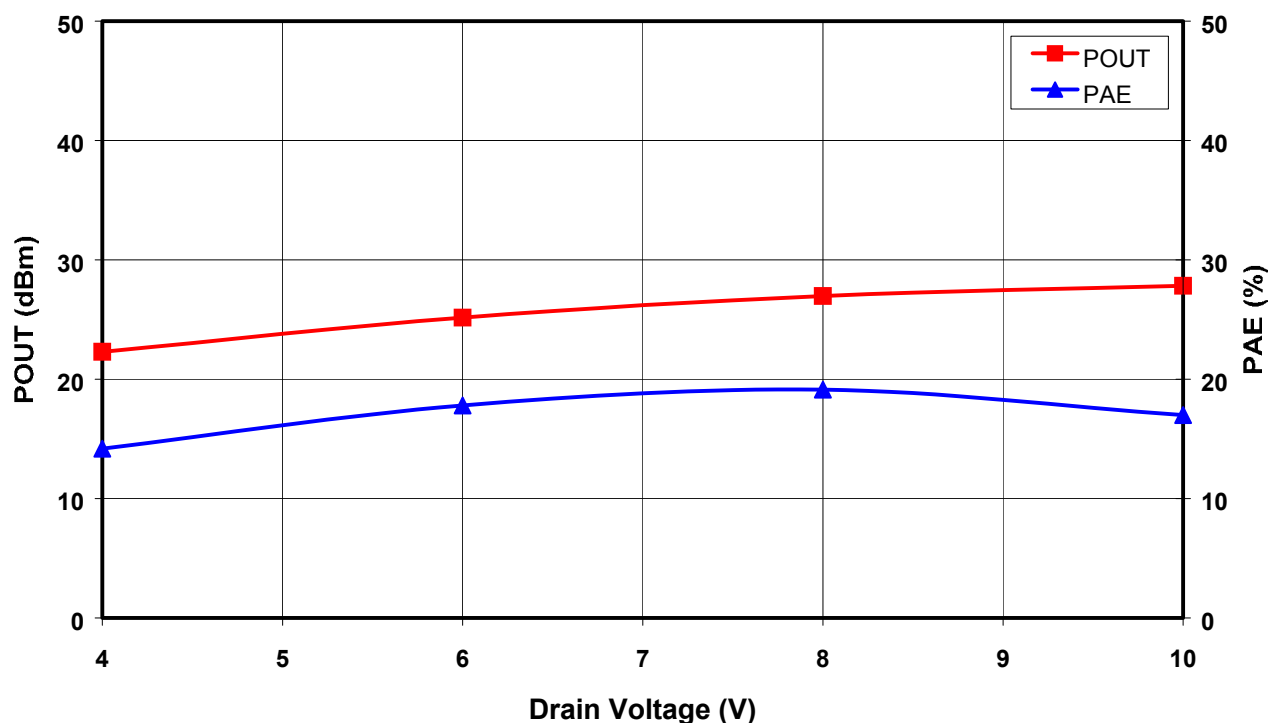
Figure 2. Saturated Output Power and Power Added Efficiency vs. Drain Voltage at f_0 = 18 GHz .
