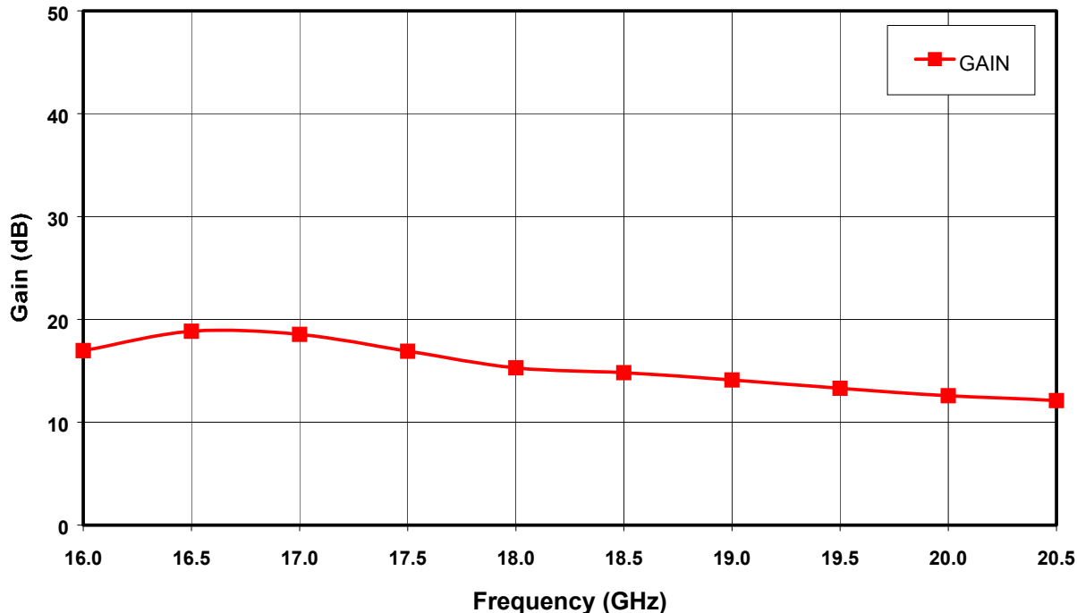
Figure 4. Small Signal Gain vs. Frequency at V_{DD} = 8V .
