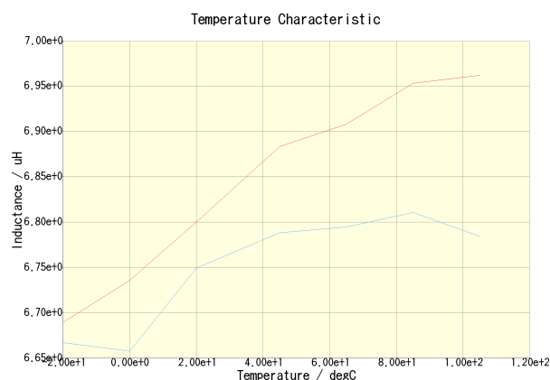
VLF403215MT-6R8M-CA(DC = 0A) VLF403215MT-6R8M-CA(DC = 0.57A)
