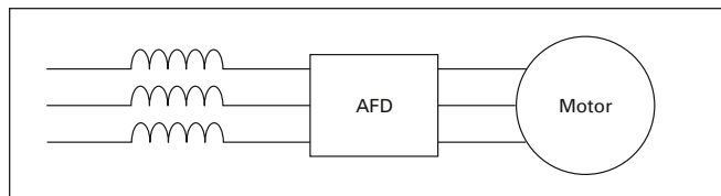
Figure 31.3-2. Line Reactor
