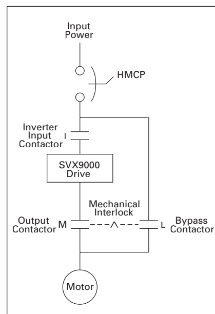
Figure 31.4-1. Power Diagram for Bypass Options RB and RA
