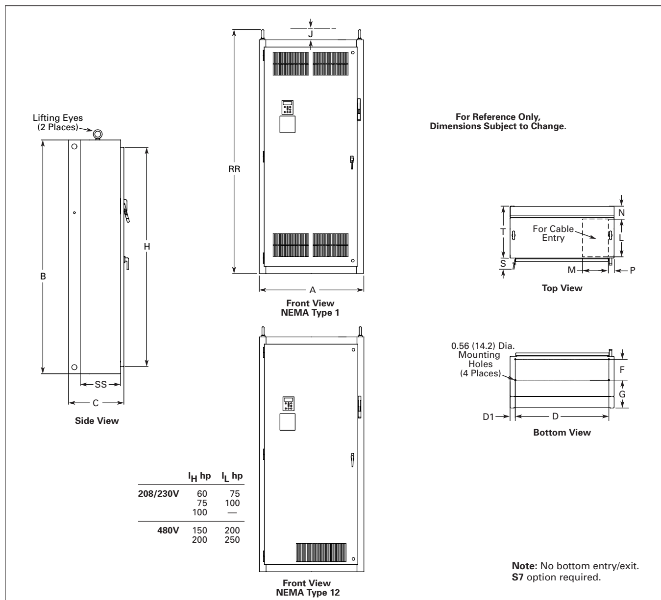
Figure 31.4-7. Approximate Dimensions
