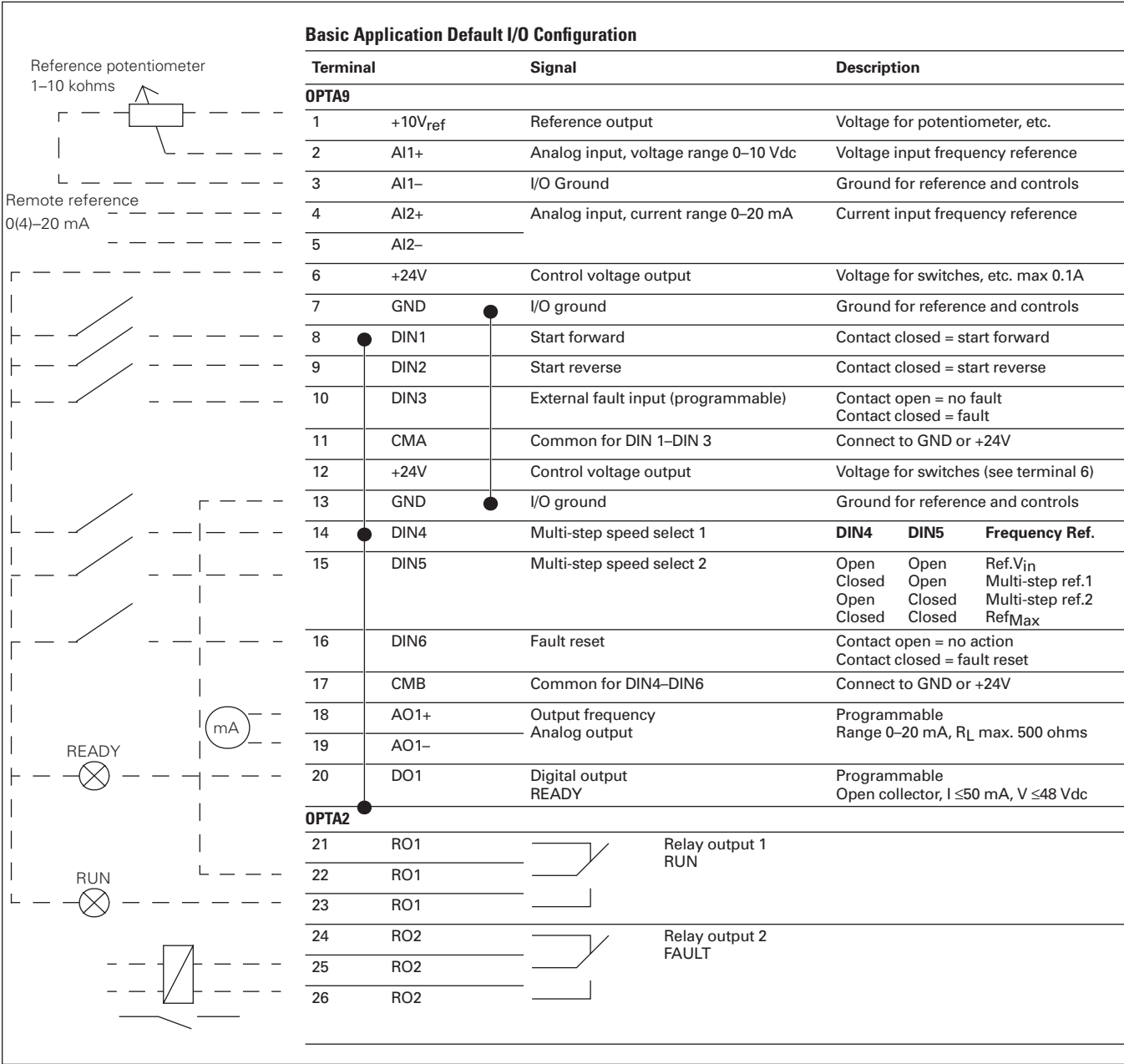
Figure 31.3-15. Control Input/Output
