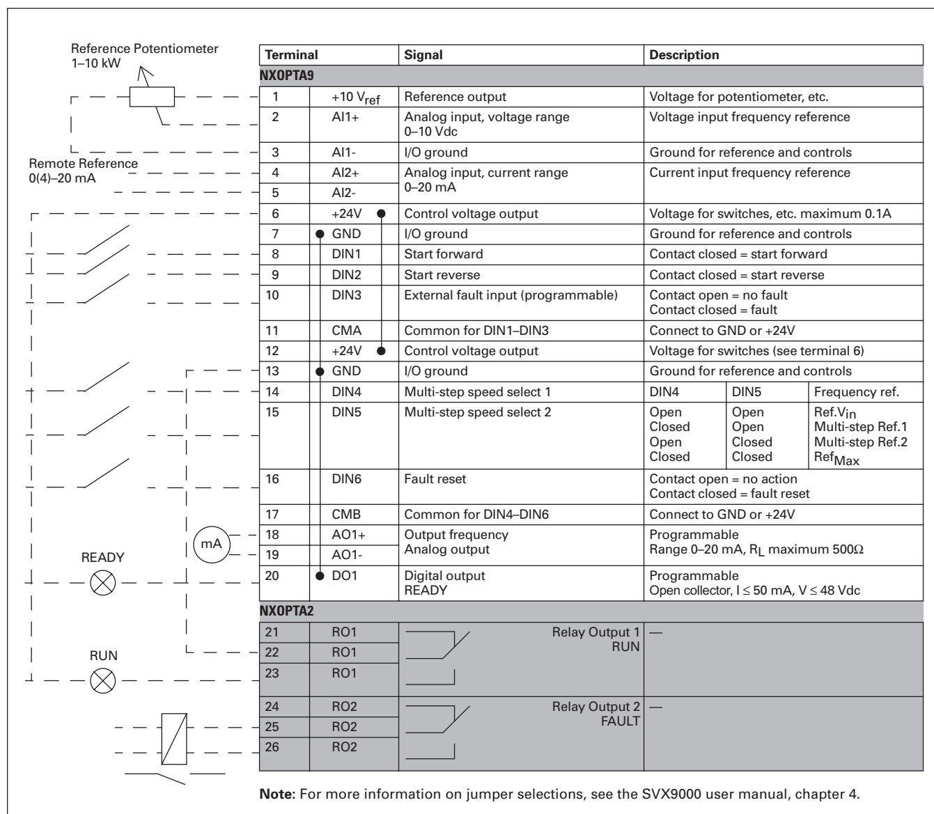
Figure 31.4-11. Basic Application Default I/O Configuration
