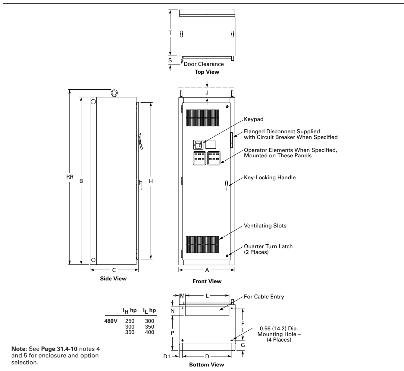
Figure 31.4-8. Approximate Dimensions
