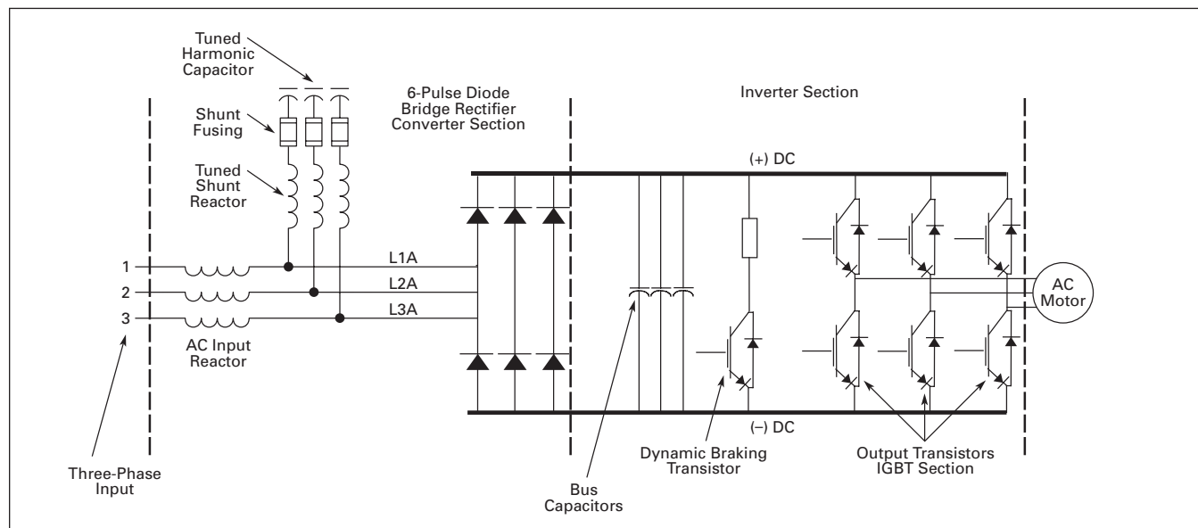
Figure 31.3-4. CFX9000 Drive with Integrated Passive Filter
