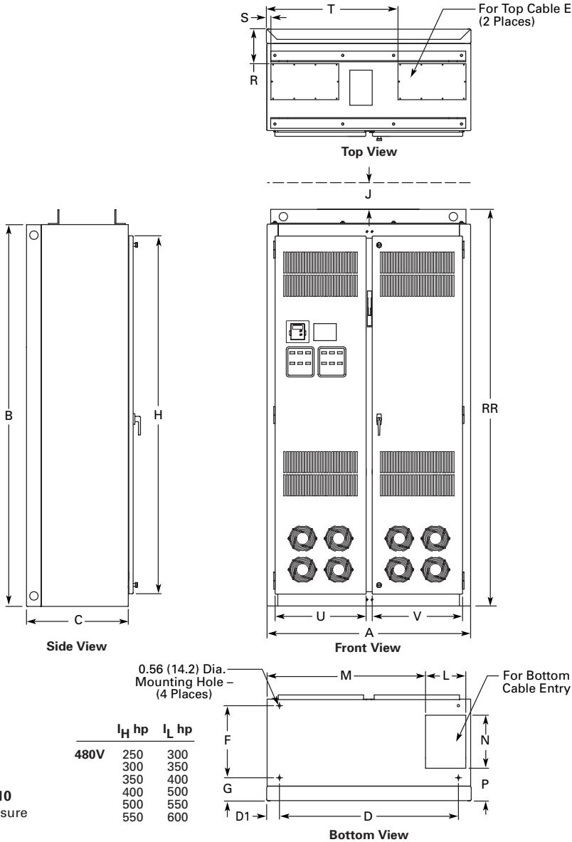
Figure 31.4-9. Approximate Dimensions
