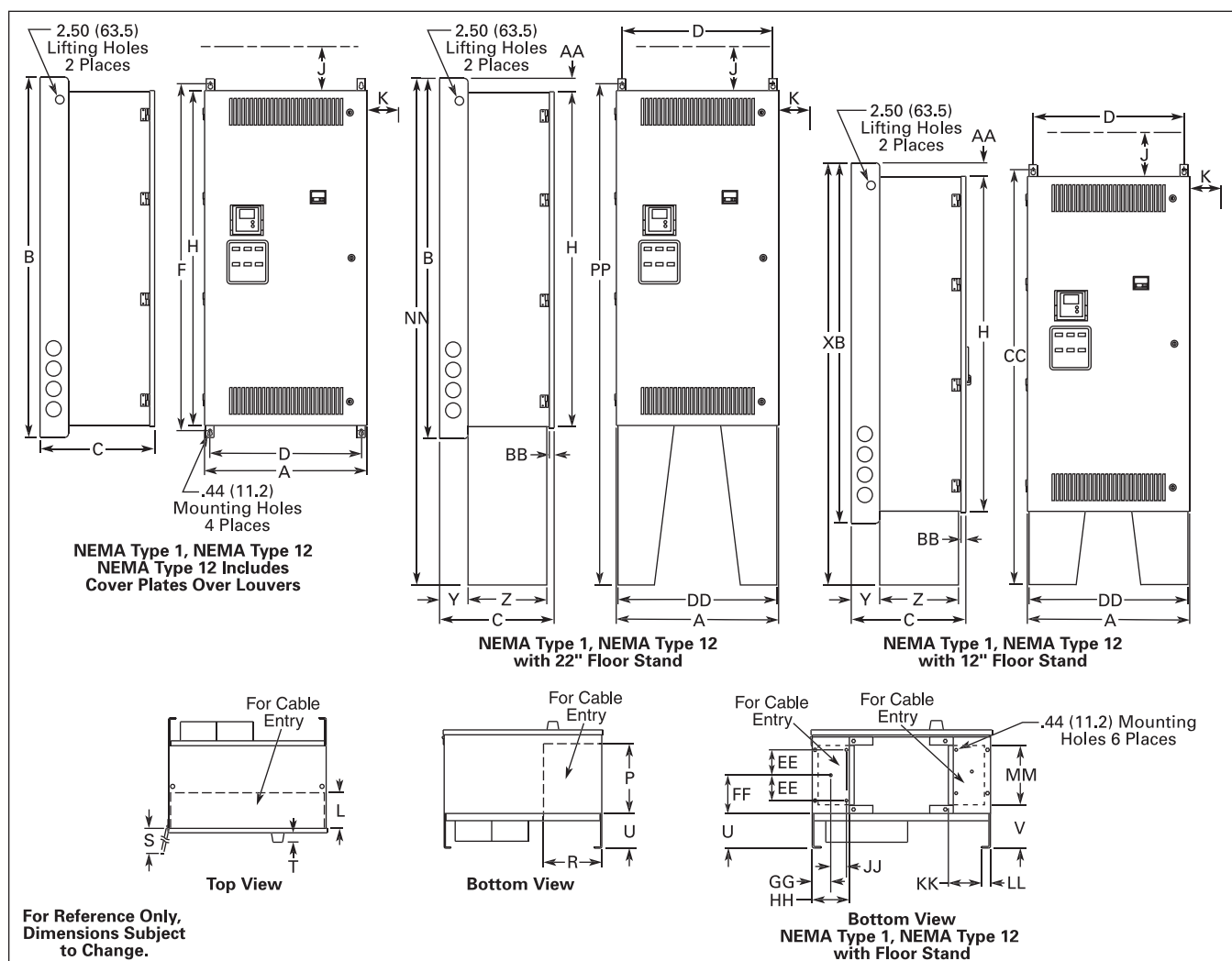
Figure 31.4-4. Approximate Dimensions
