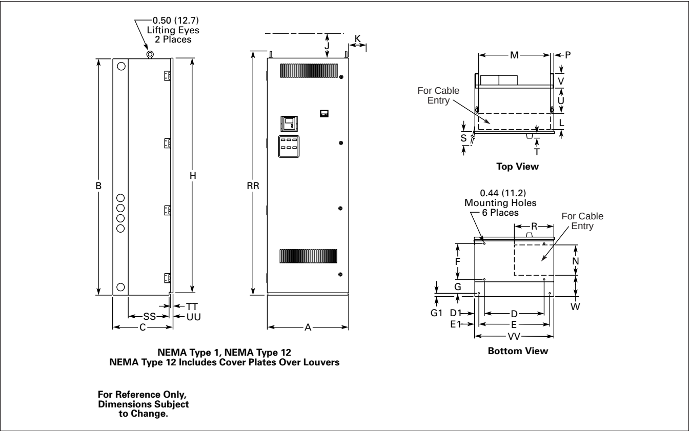
Figure 31.4-5. Approximate Dimensions
