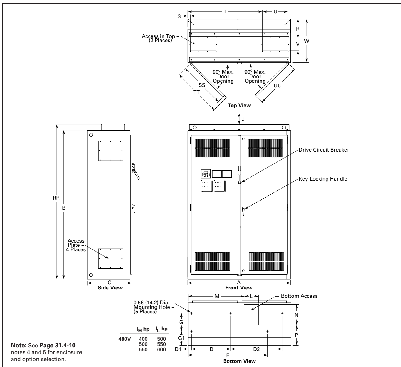
Figure 31.4-10. Approximate Dimensions
