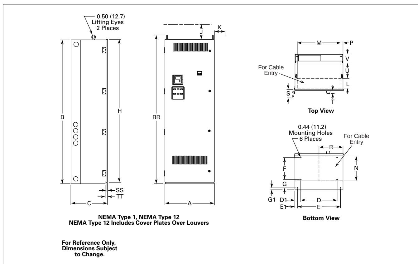
Figure 31.4-6. Approximate Dimensions
