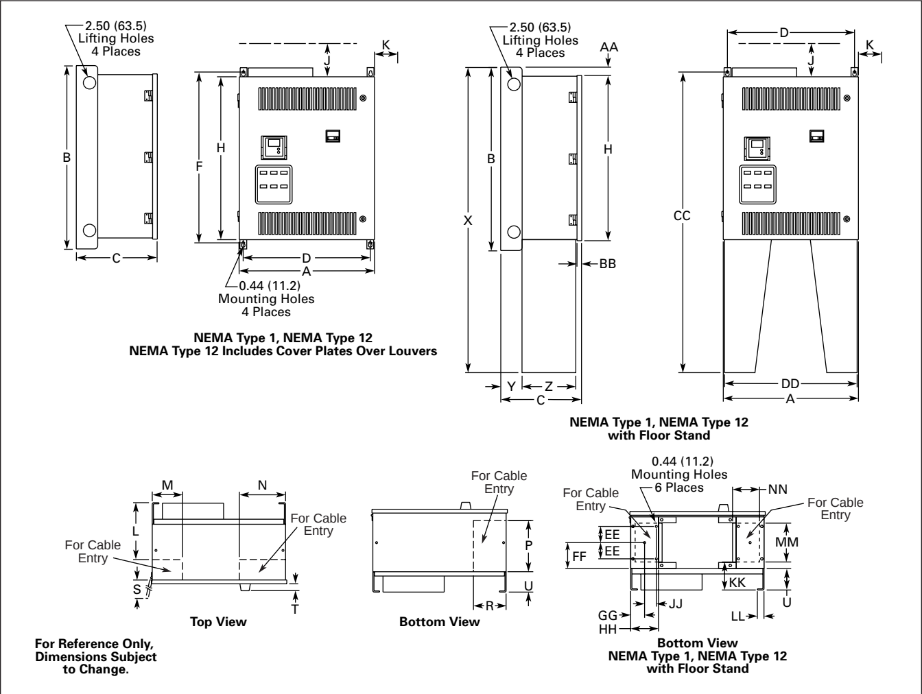
Figure 31.4-3. Approximate Dimensions
