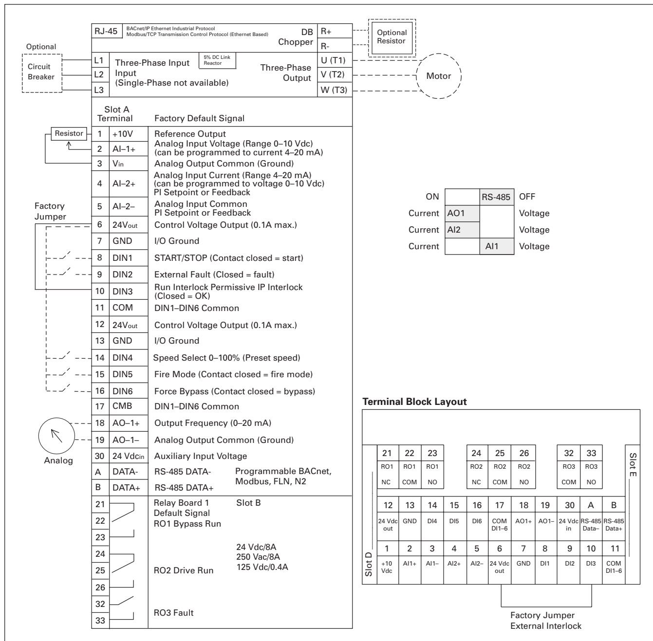
Figure 31.5-1. Control Input/Output, PID Application
