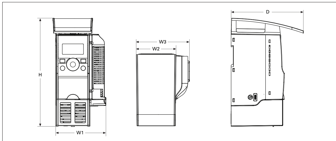
Figure 31.1-3. NEMA 1/IP21 M-Max Drives and Communication Adapter Kit
