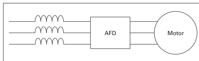
Figure 31.2-7. Line Reactor
