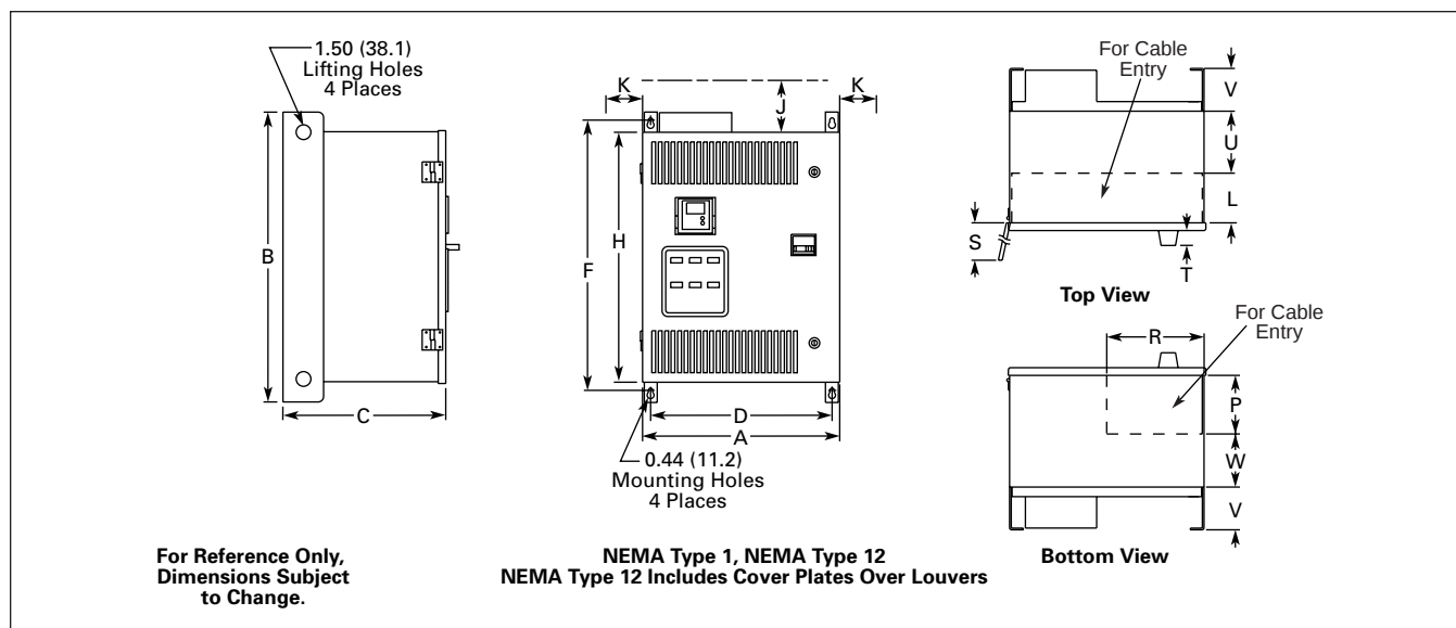
Figure 31.4-2. Approximate Dimensions
