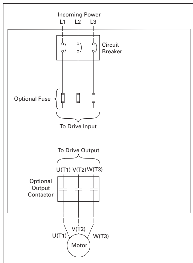
Figure 31.5-6. H-Max Series IntelliDisconnect Power Wiring
