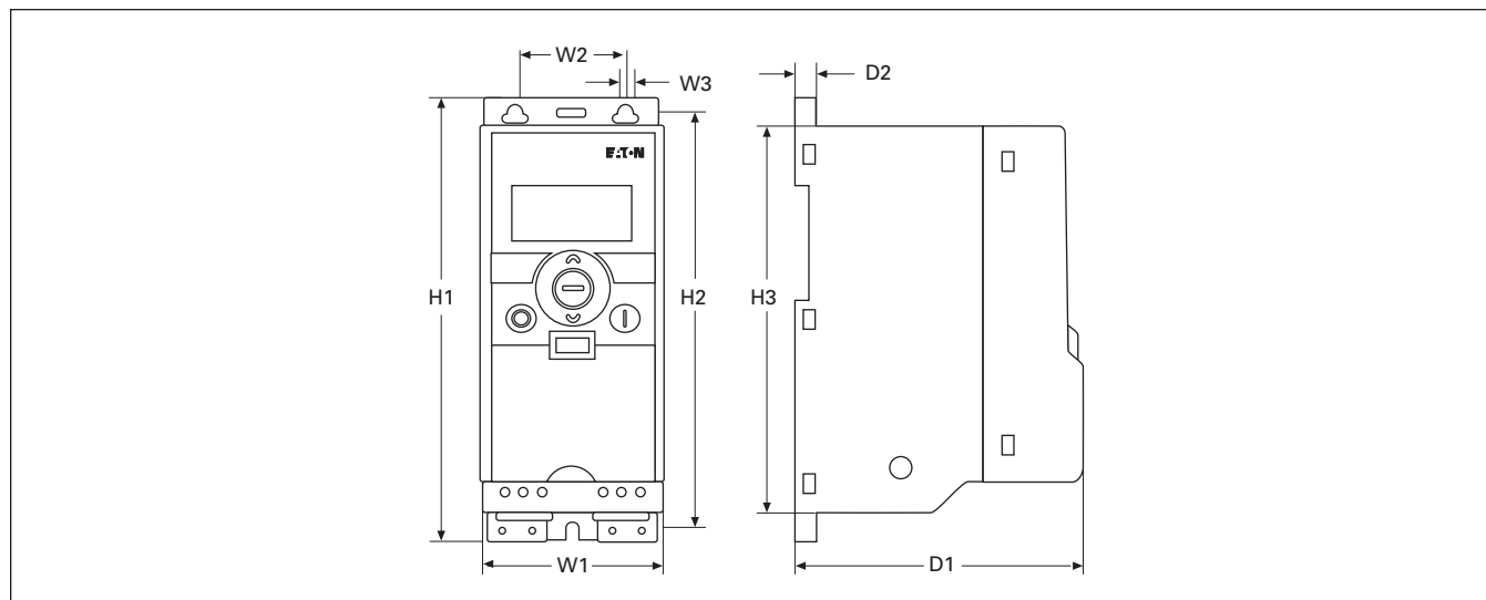
Figure 31.1-2. M-Max Drives
