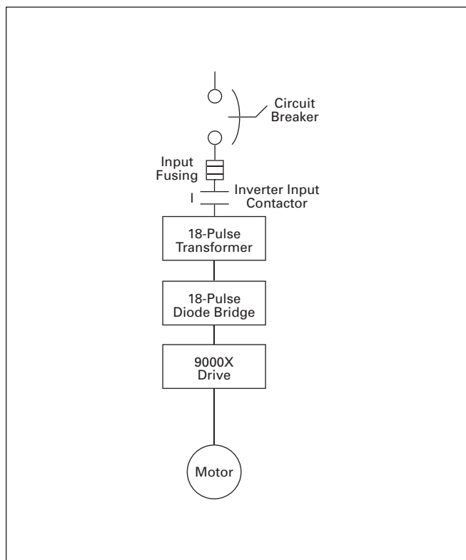
Figure 31.2-14. Power Diagram 25–250 hp I_L and 25–200 hp I_H
