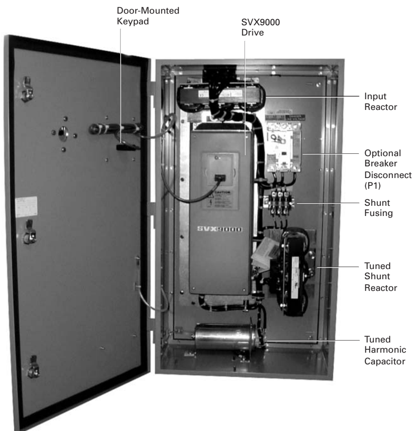
CFX9000 Drive—UL Type 12, 40 hp
