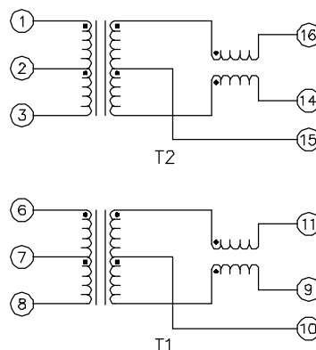
SCHEMATIC
