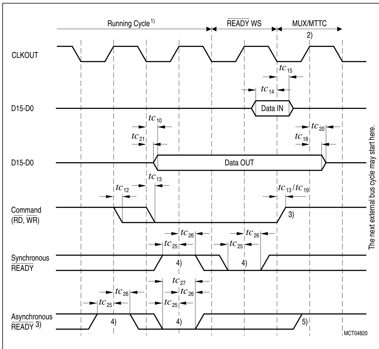
Figure 21 \overline{\text{READY}} Timing
