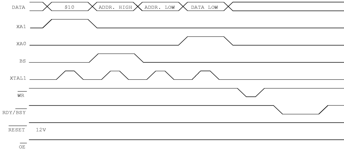
Figure 63. Programming the Flash Waveforms
