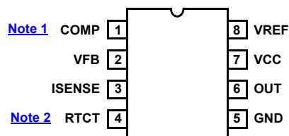
IS7-1845ASRH, IS7-1845ASEH (8 LD CDIP2-T8 SBDIP) TOP VIEW
