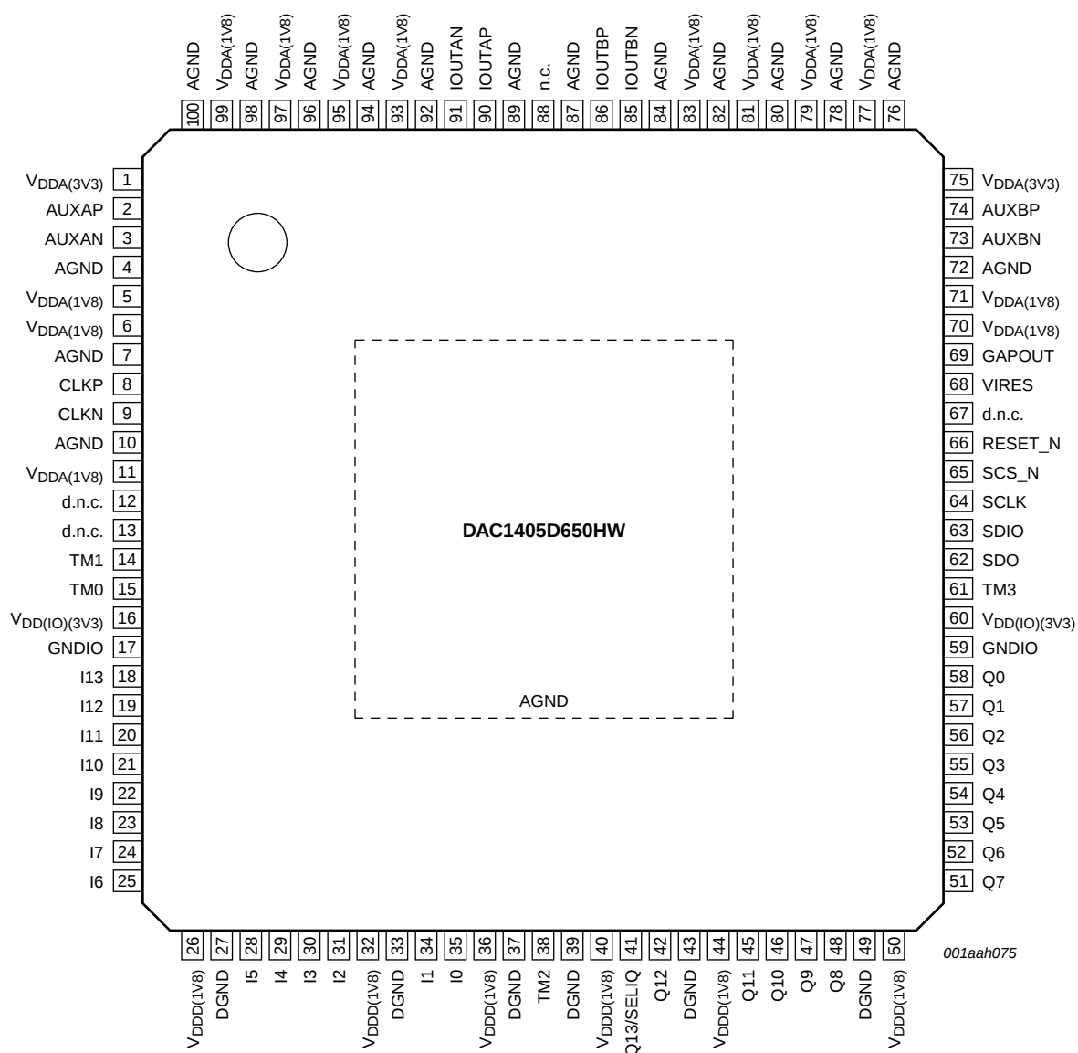
Fig 2. Pin configuration
