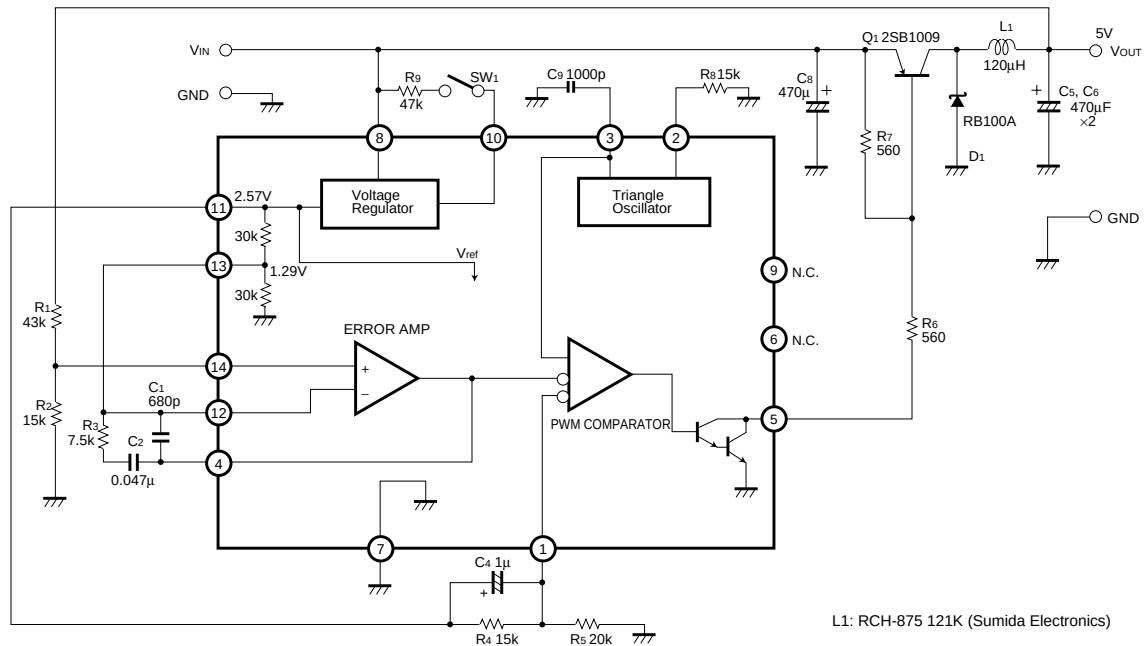
Fig.2 Step-down converter
