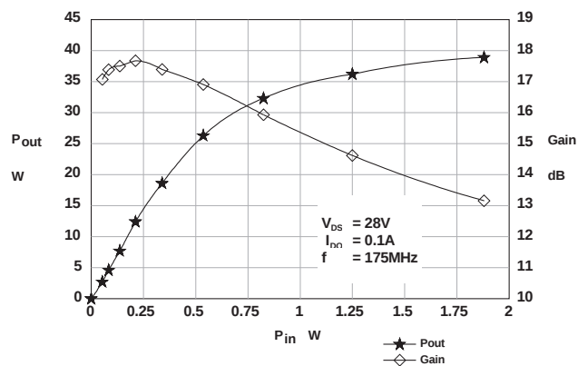
Figure 2 – Power Output & Gain vs. Power Input.
