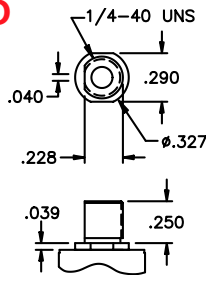
THREADED
