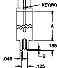
FRONT VIEW SINGLE POLE
