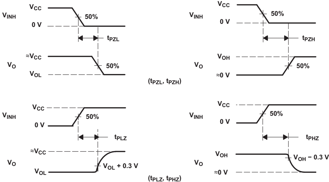
VOLTAGE WAVEFORMS
