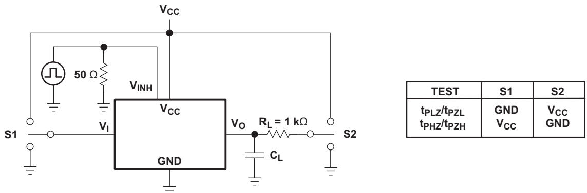
TEST CIRCUIT
