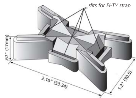
El-Ty Spacer
