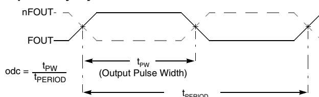
Figure 7: Output Duty Cycle
