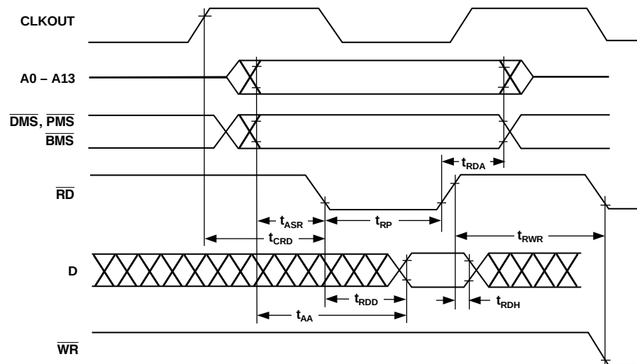
Figure 32. Memory Read
