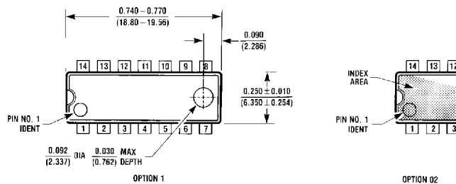
14-Lead Ceramic Dual-In-Line Package (J) Order Number 54164DMQB Package Number J14A
