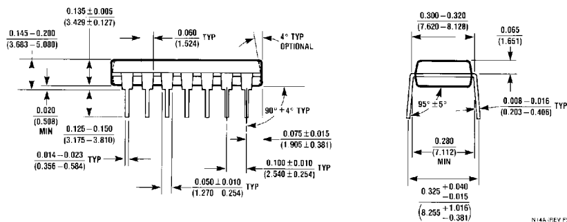
14-Lead Molded Dual-In-Line Package (N) Order Number DM74164N Package Number N14A
