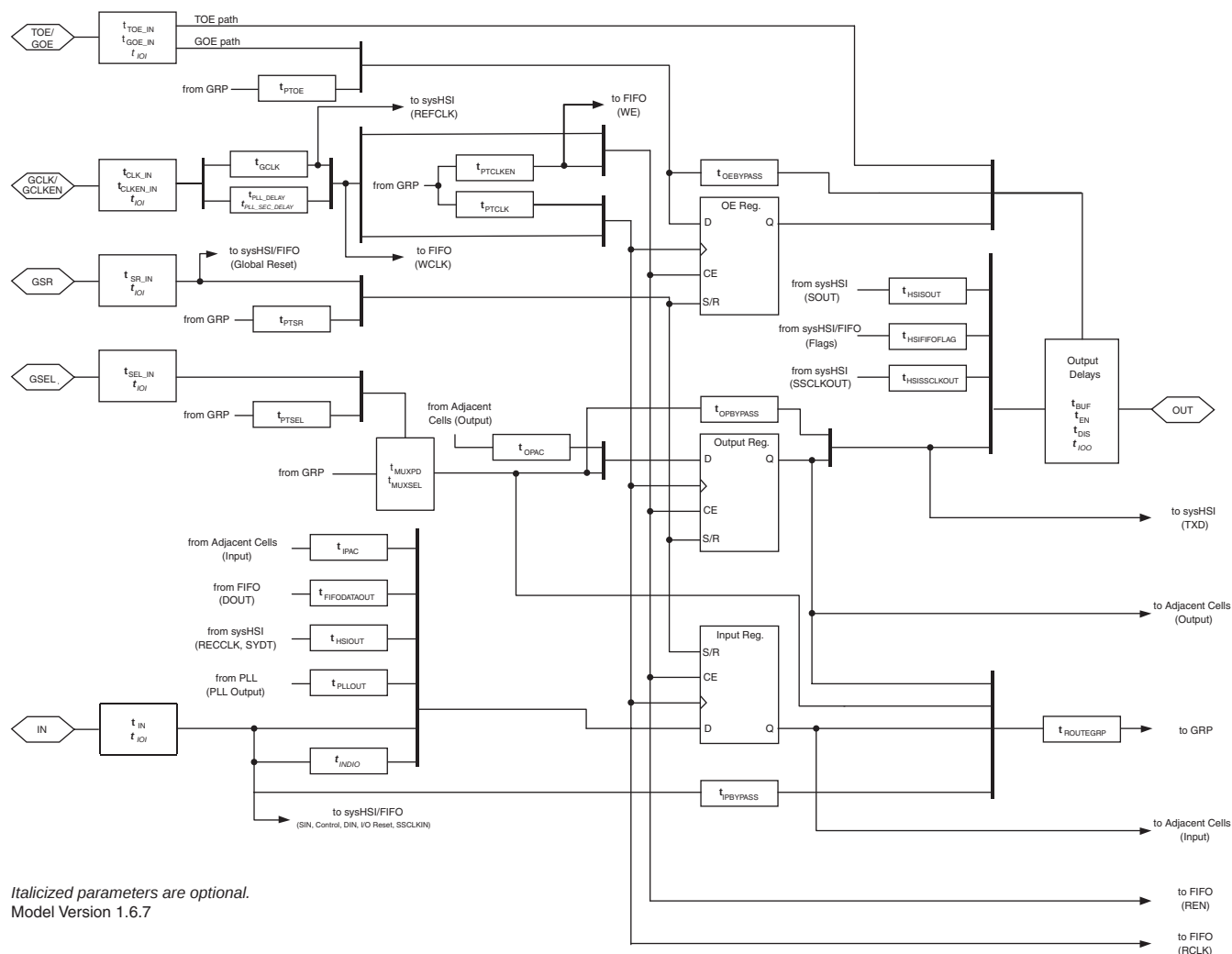
Figure 16. ispGDX2 Timing Model Diagram (I/O Cell)
