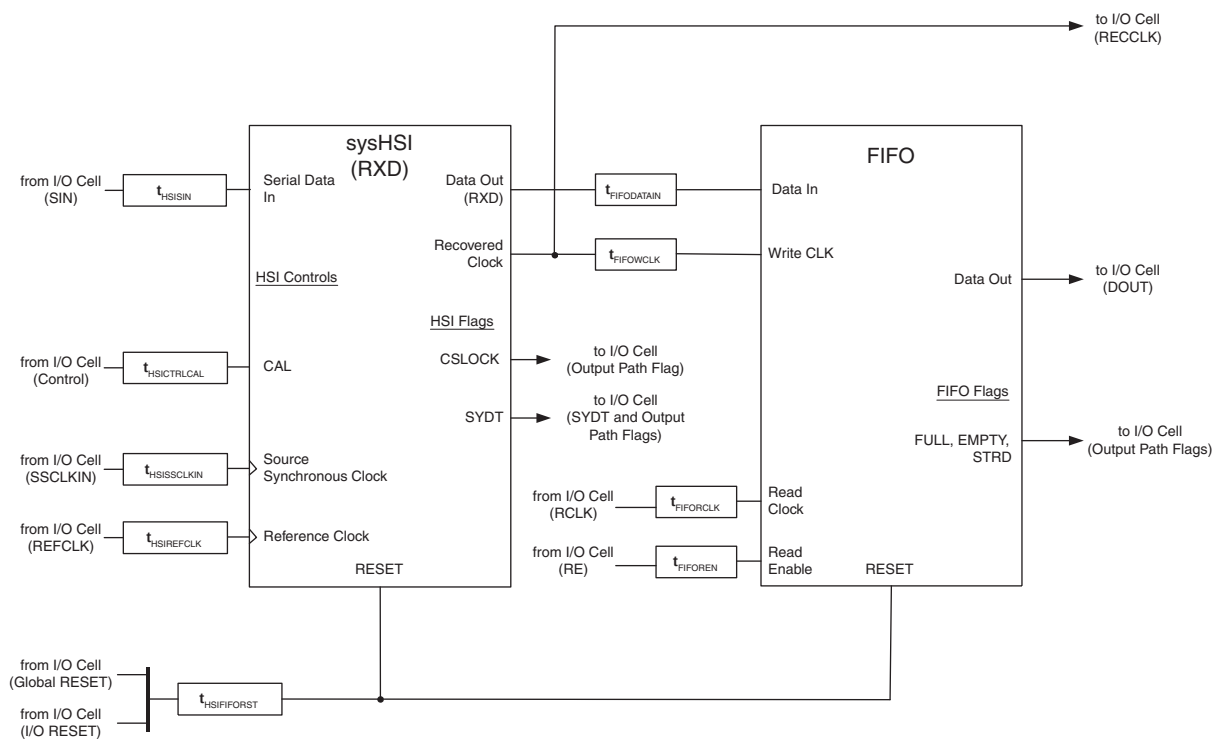
Figure 17. ispGDX2 Timing Model Diagram (with sysHSI and FIFO Receive Mode)
