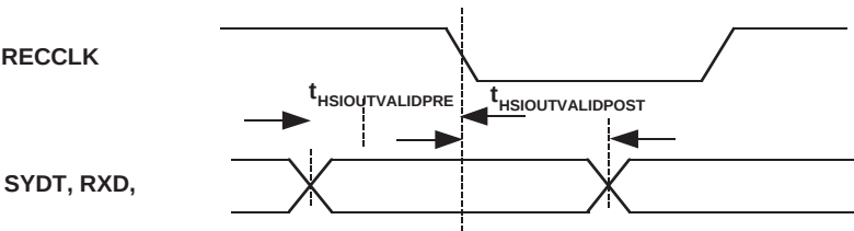
INTERNAL TIMING FOR sysHSI BLOCK
