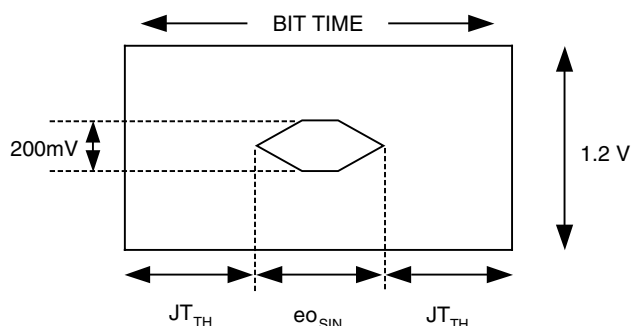
Figure 20. Receive Data Eye Diagram Template (Differential)
