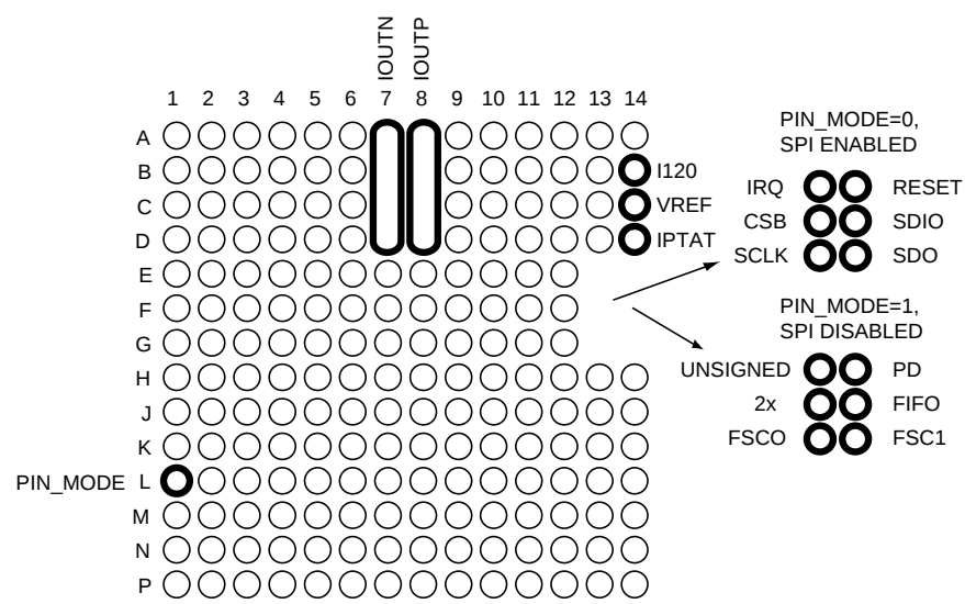
Figure 6. AD9736 Analog I/O and SPI Control Pins (TOP view)
