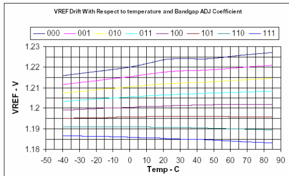
Figure 31. BANDGAP Temperature Characteristic for Various TRMBG Values
