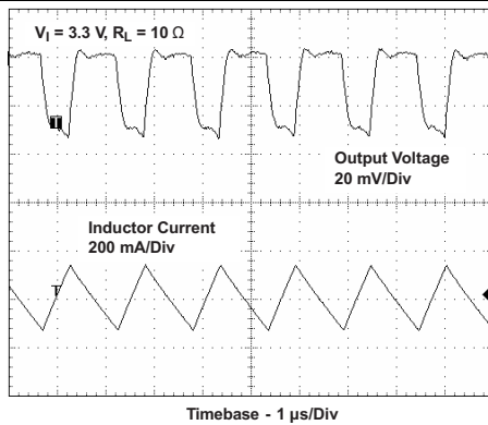
Figure 15. Output Voltage in Continuous Mode
