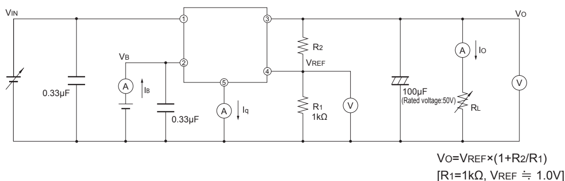
Fig.2 Test Circuit for Ripple Rejection (1)
