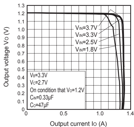
Fig.5 Overcurrent Protection Characteristics (PQ015YZ5MZxH)
