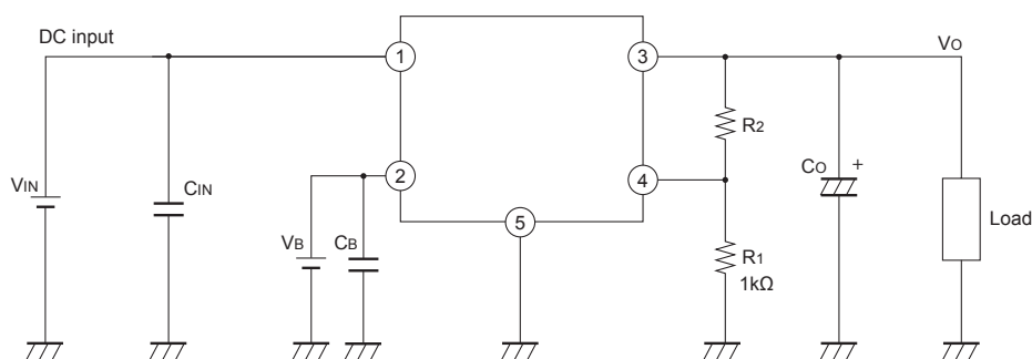
Fig.22 Typical Application
