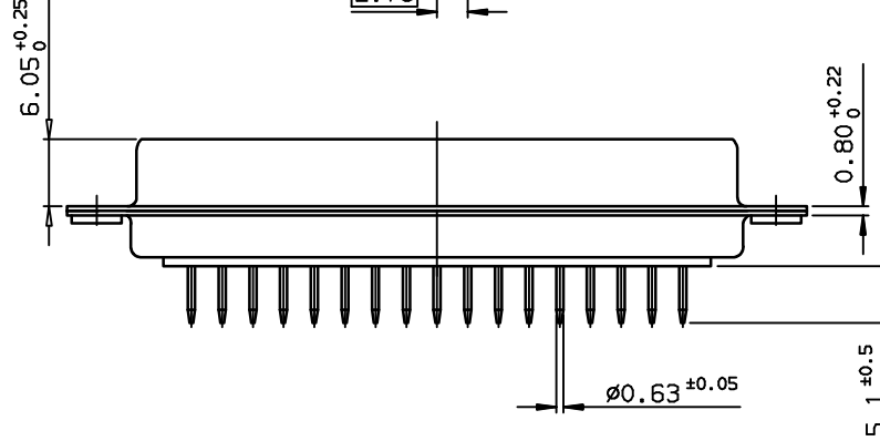
LAYOUT DIMENSIONS (after plating) CONNECTOR SIDE VIEW
