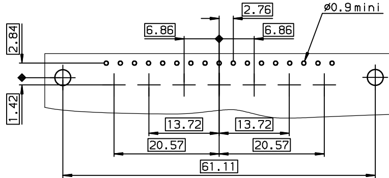
LAYOUT DIMENSIONS (after plating) CONNECTOR SIDE VIEW
