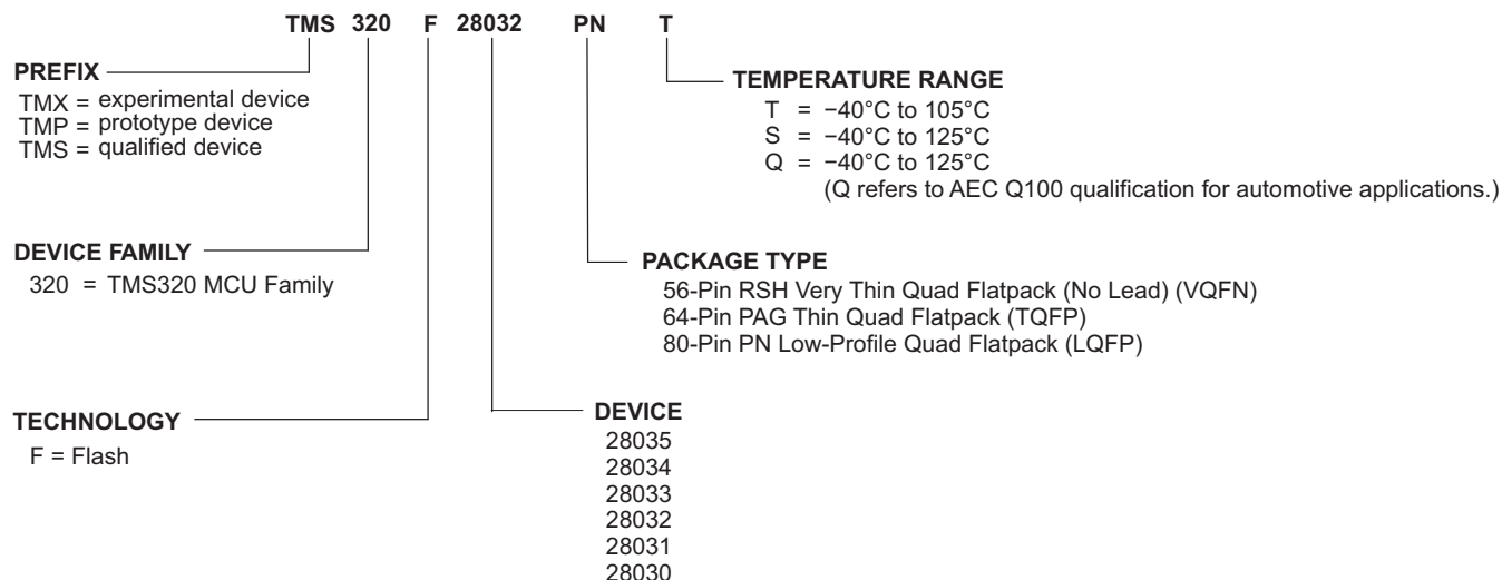
Figure 8-1. Device Nomenclature
