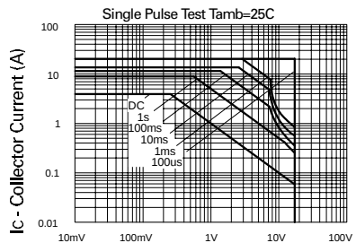
V_{CE} - Collector Voltage
