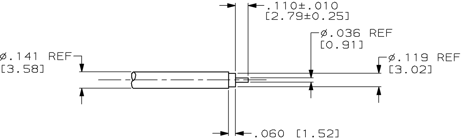
RECOMMENDED STRIP LENGTH SCALE 2:1
