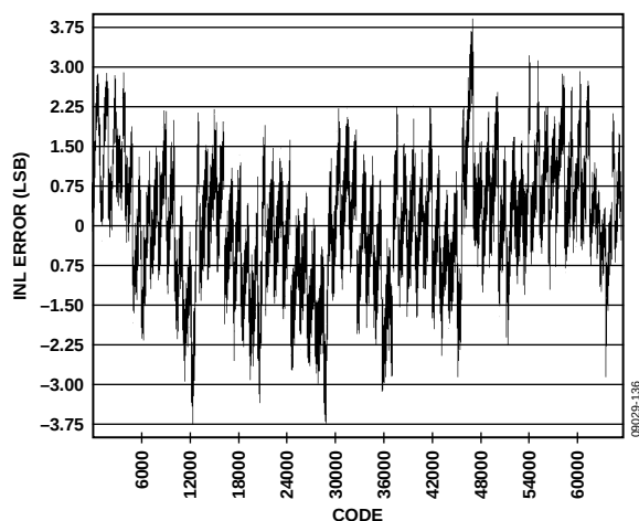
Figure 36. INL, f_{IN} = 4.3 MHz, 2.5 V p-p FS, AD9467-200
