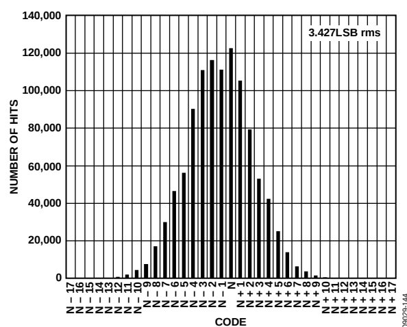
Figure 44. Input-Referred Noise Histogram, 2.5 V p-p FS, AD9467-200
