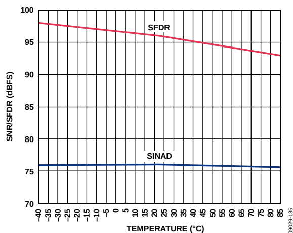
Figure 35. SINAD/SFDR vs. Temperature, f_{IN} = 97.3 MHz, 2.5 V p-p FS, AD9467-250
