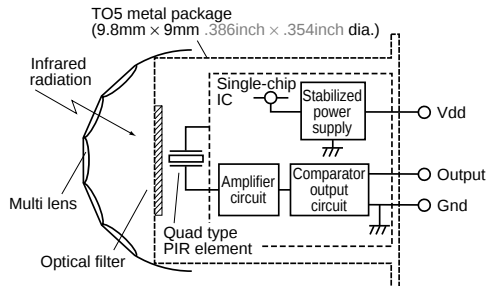
MP motion sensor block diagram
