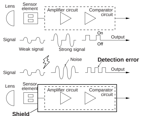
(Block diagram for a typical passive infrared sensor)
