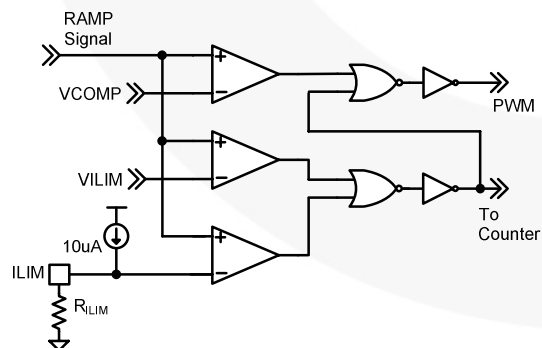
Figure 32. ILIM Network
