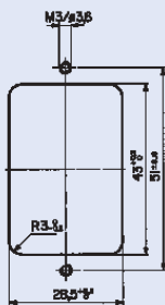
Panel cut-out
