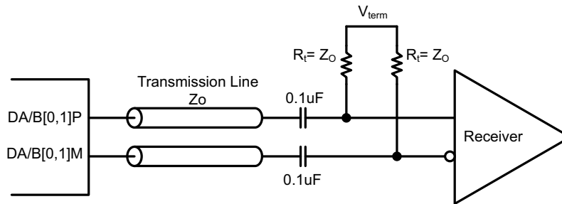
Figure 64. CML Output Connections
