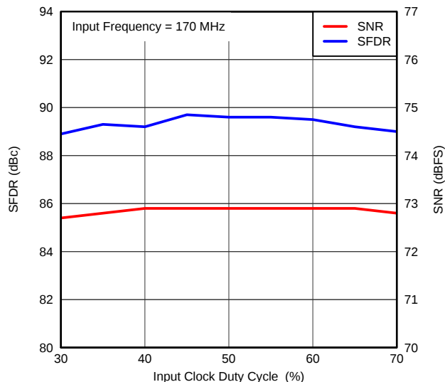
Figure 35. PERFORMANCE vs CLOCK DUTY CYCLE (170 MHz)
