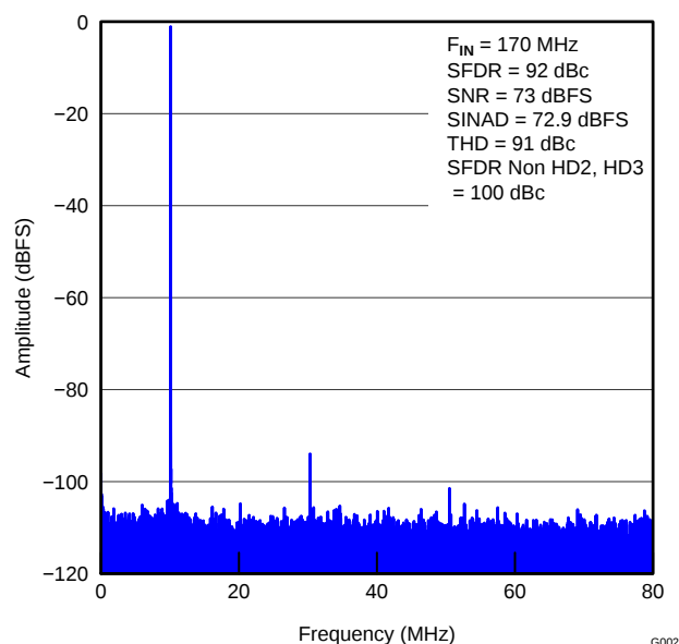
Figure 7. FFT FOR 170-MHz INPUT SIGNAL
