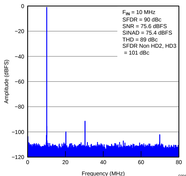
Figure 9. FFT FOR 10-MHz INPUT SIGNAL ( 2.5\text{-V}_{PP} Full-Scale)
