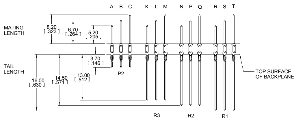
CONTACT OVERVIEW
