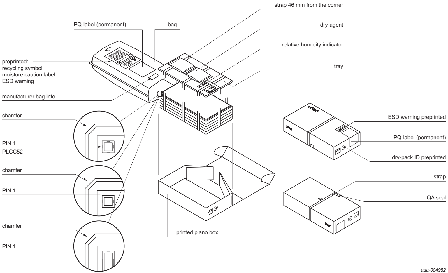
Fig 36. Packing information 5 tray
