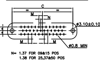
PCB DRILLING DETAIL - 50 POS
