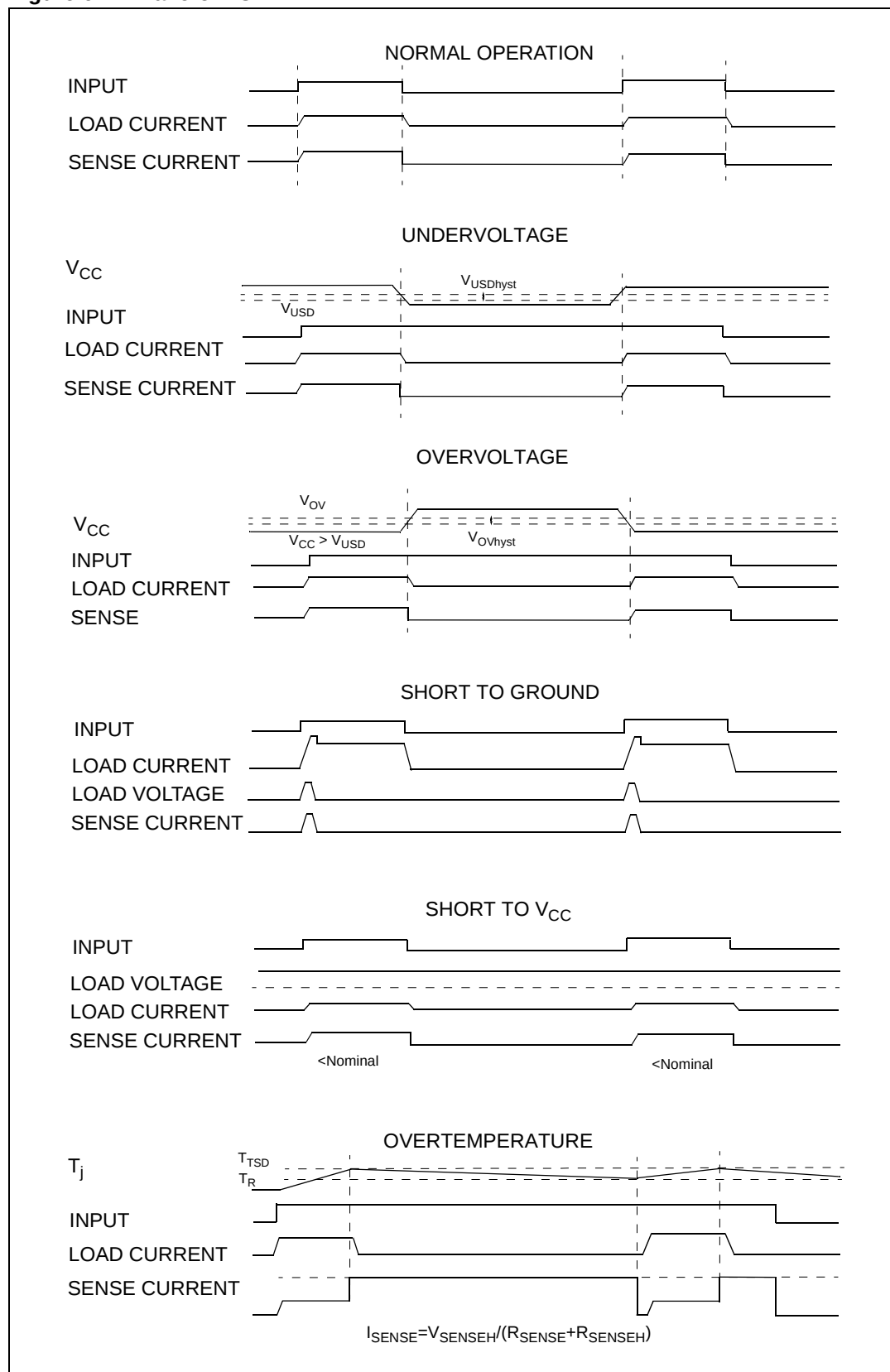
Figure 6. Waveforms
