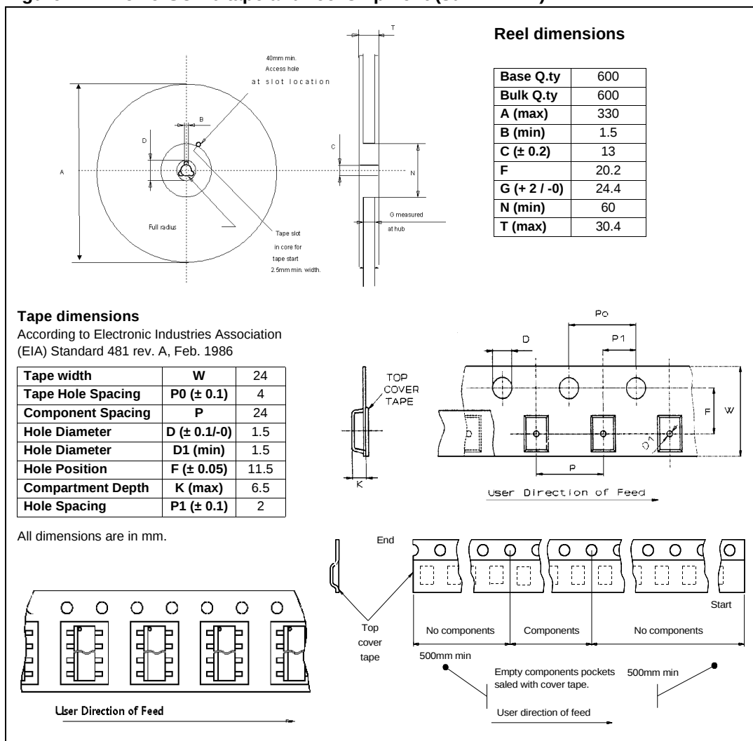
Figure 27. PowerSO-10 tape and reel shipment (suffix "TR")
