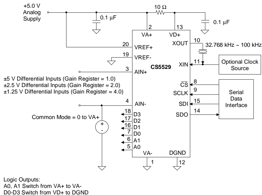
Figure 10. CS5529 Configured with a +5.0\text{ V} Analog Supply.
