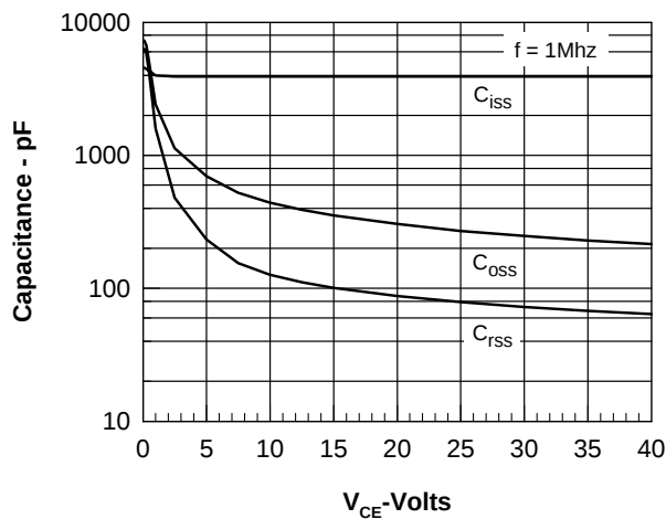
Figure 6. Capacitance Curves
