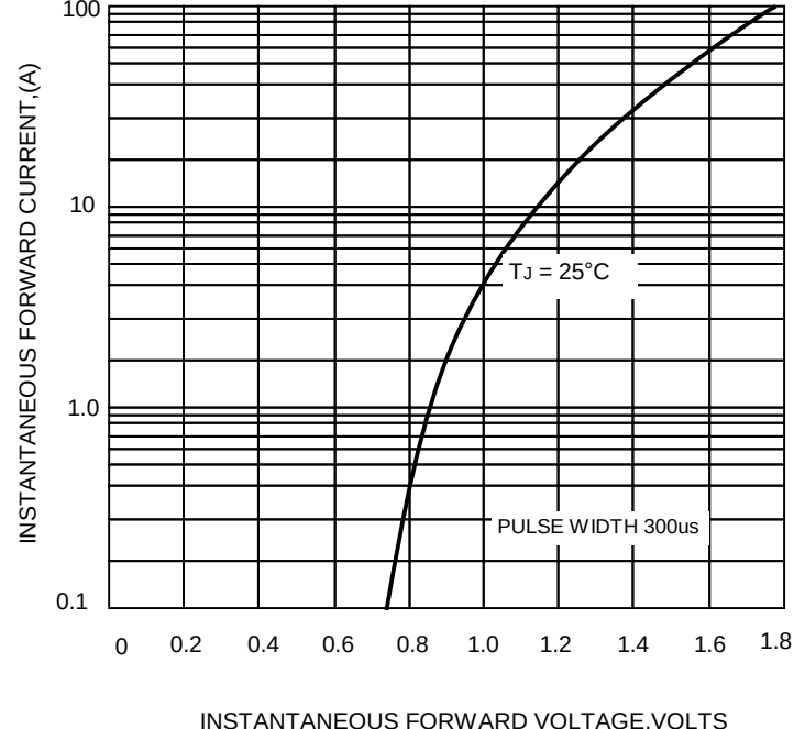
FIG.4-TYPICAL FORWARD CHARACTERISTICS
