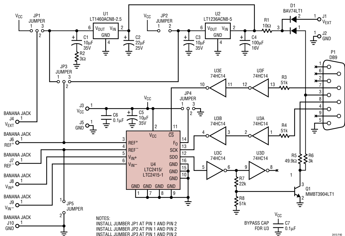
Figure 40. 24-Bit A/D Demo Board Schematic
