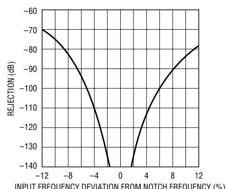
Figure 32. Rejection vs Frequency at V_{IN}
