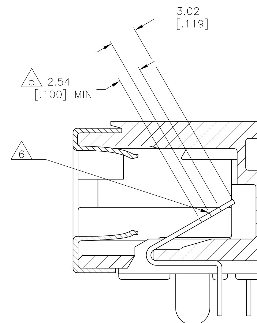
SECTION J-J
