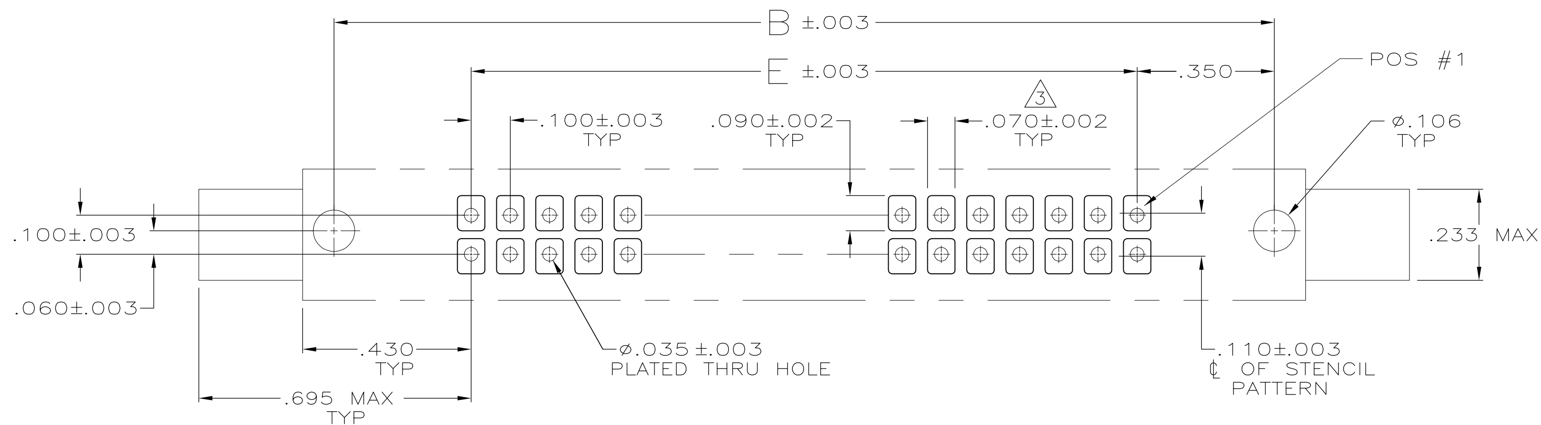
RECOMMENDED P C BOARD MOUNTING DIMENSIONS
