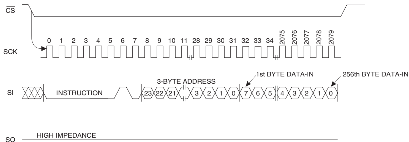
Figure 9. PROGRAM Timing
