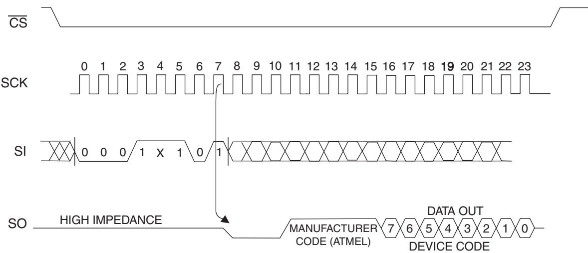
Figure 13. RDID Timing
