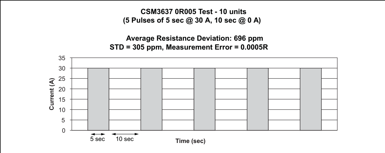
FIGURE 6 - PULSE TEST I
