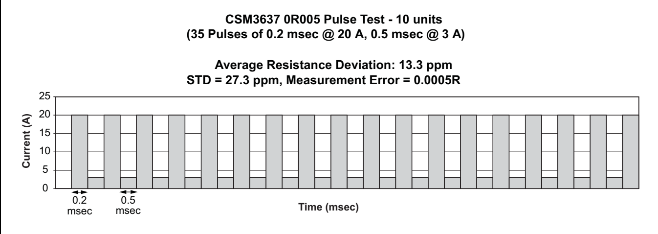
FIGURE 7 - PULSE TEST II
