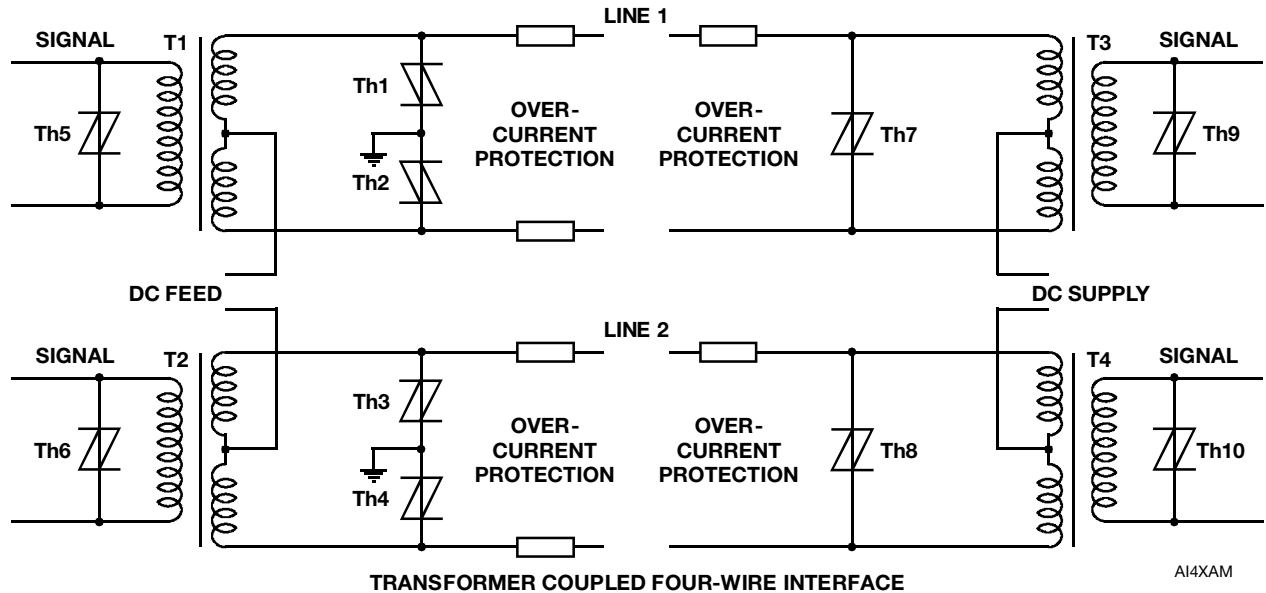
Figure 7. 4-Wire System
