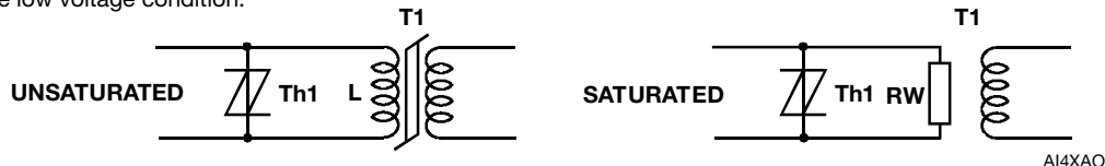
Figure 4. Transformer Saturation
