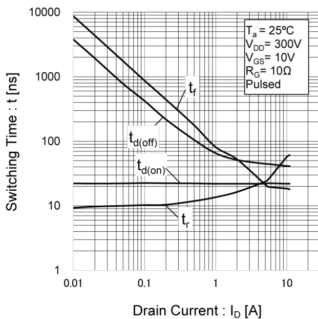
Fig.14 Switching Characteristics
