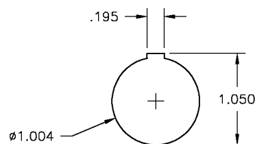
BACKEND DIMS. OF RECEPTACLE
