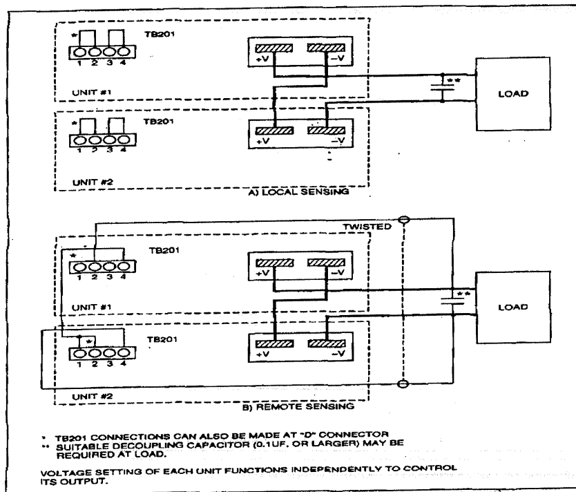
FIGURE 7: SERIES OPERATION
