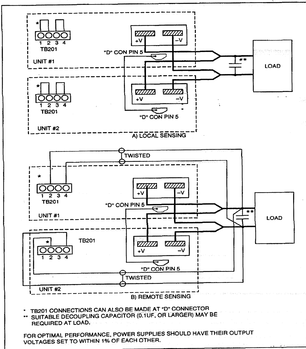
FIGURE 6: PARALLEL OPERATION
